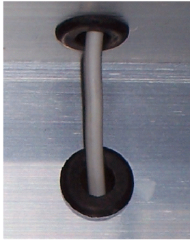
Grommets keep wires from rubbing on the aluminum and being cut.
