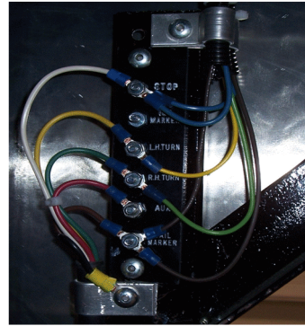
Easy to read hitch setup.
